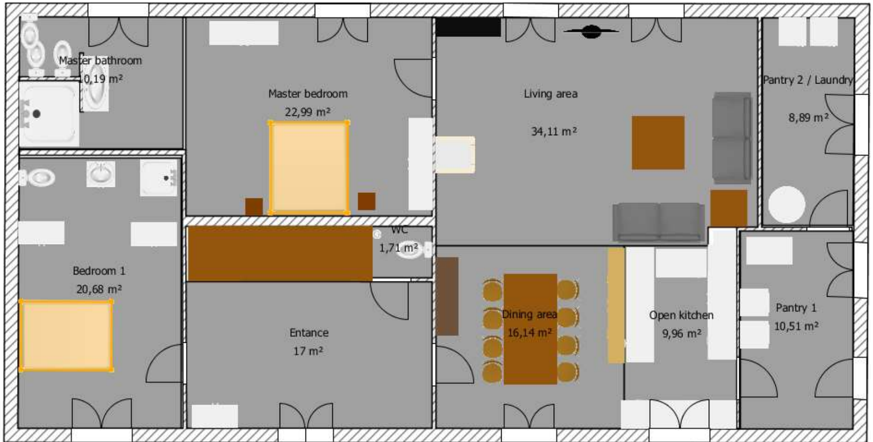
Ground floor 18 x 9 m
